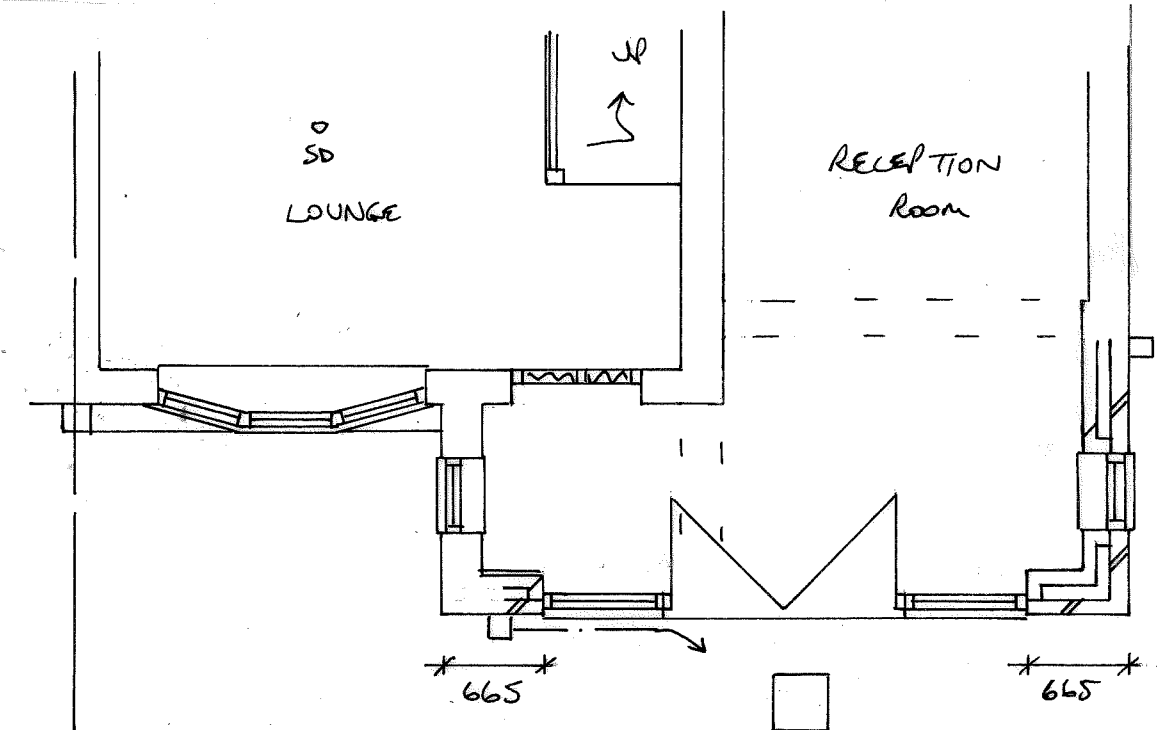
PROPOSED GROUND FLOOR PLAN 1:50
