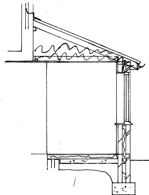
SECTION 1:50
